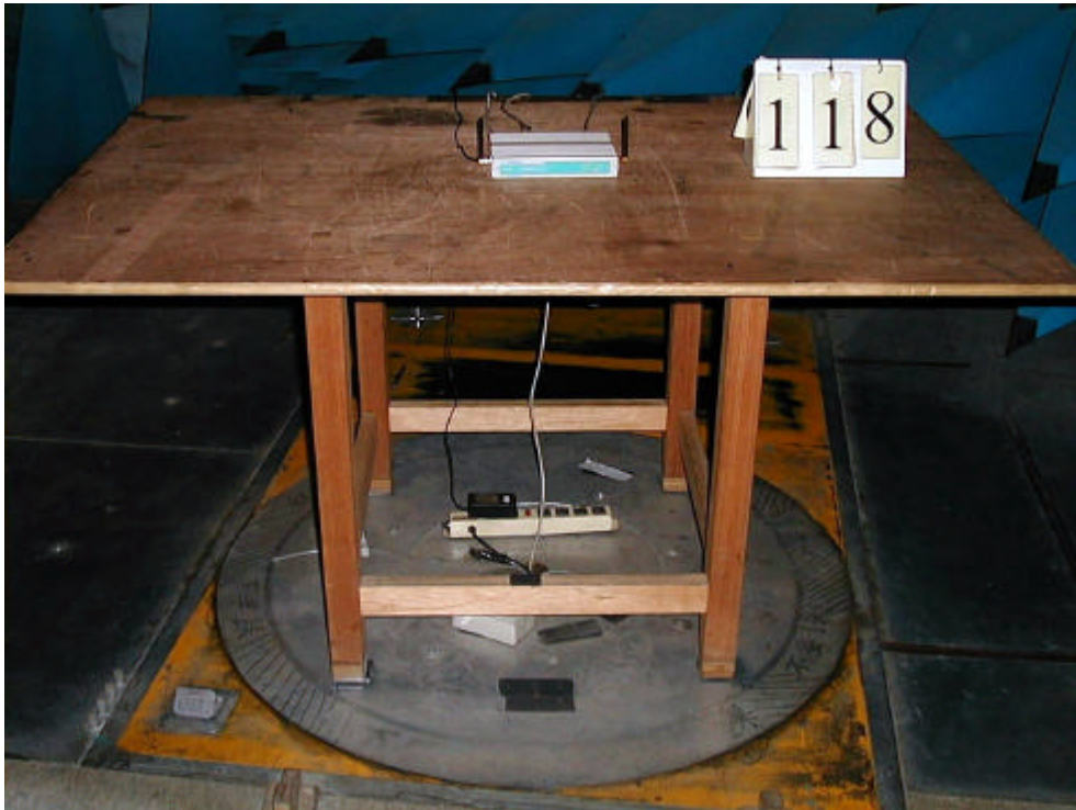
Pig 1 Front View of the Test Configuration for AC/DC Adaptor
