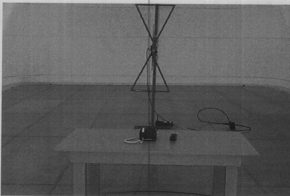
Radiated Emission Test Set-up - Front View
