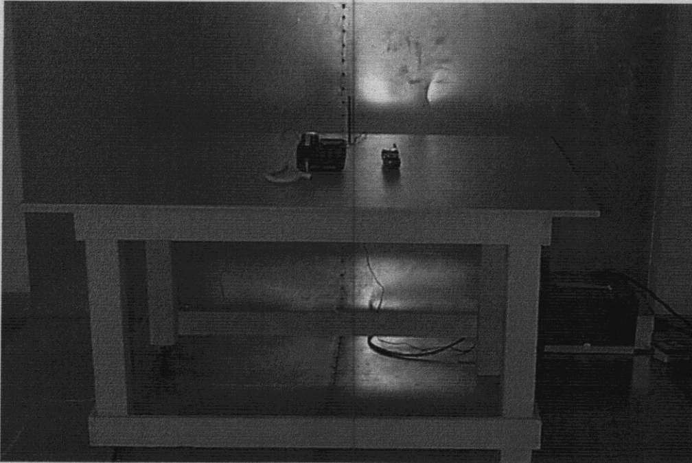
Conducted Emission Test Set-up - Front View
