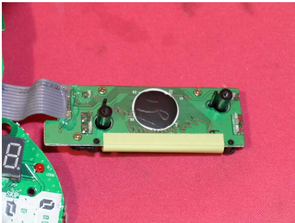
LCD display PCB rear side
