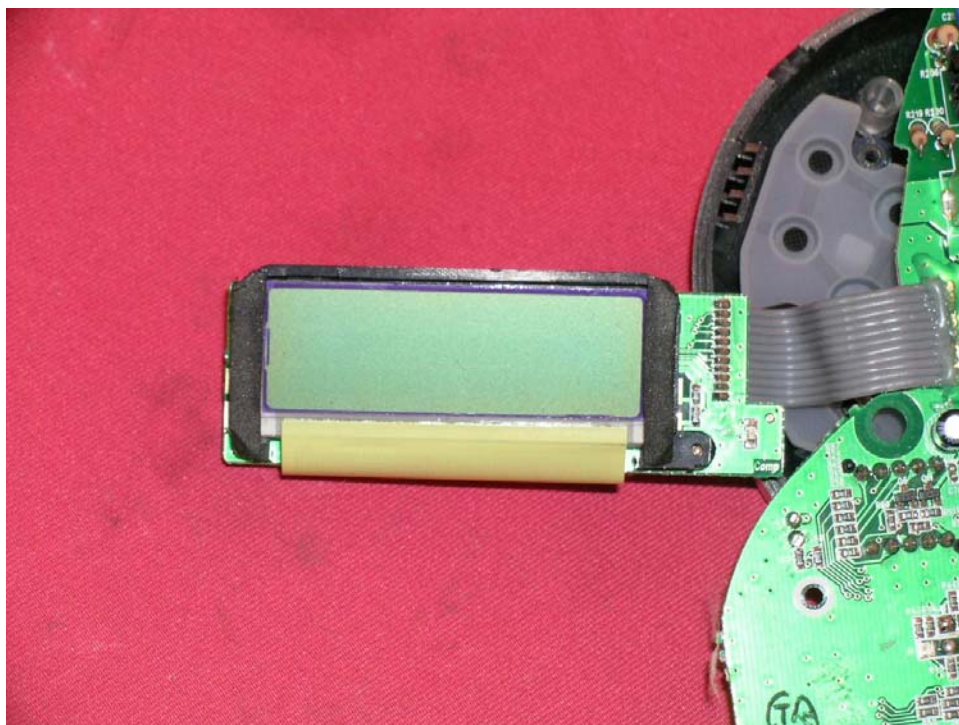
LCD display PCB front side
