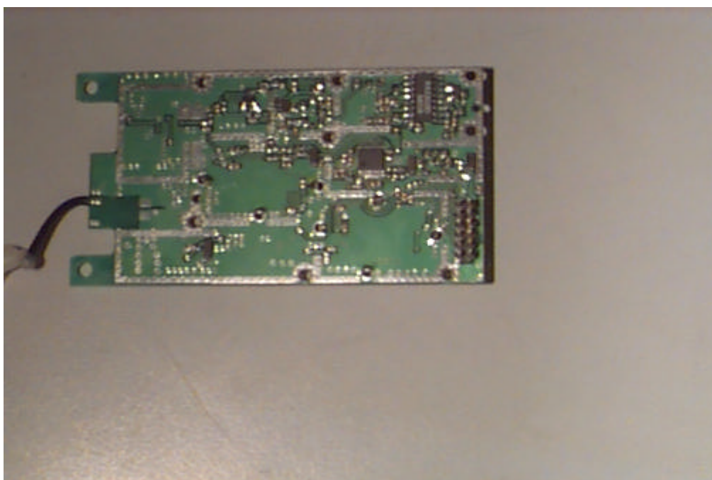
Base Transceiver Board - Solder Side
