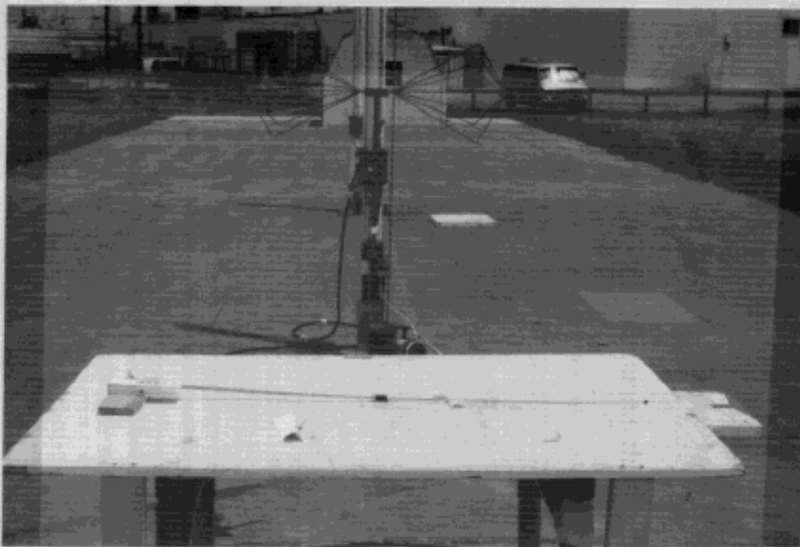
Photograph 4 Radiated Emissions - Rear View Typical 4.1.2A Test Setup
