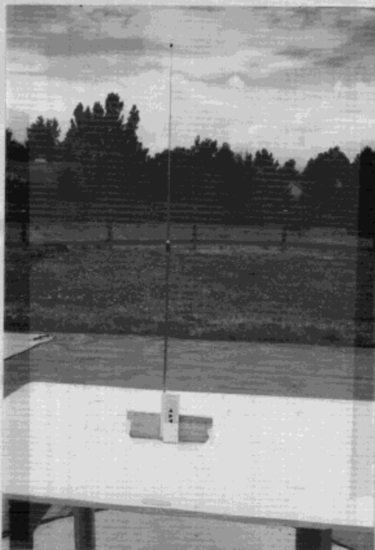
Photo 1 Radiated Emissions Close-Up Front View Vertical Polarization
