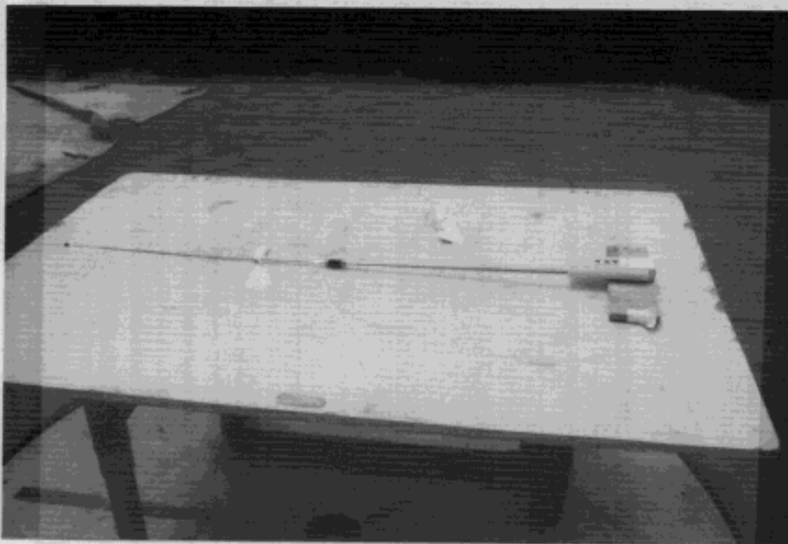
Photo 5 Radiated Emissions - Close-up Front View Horizontal Polarization
