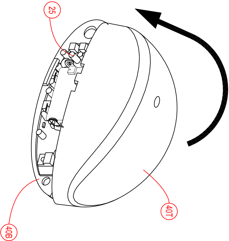
3a. CLOSE COVER AS SHOWN IN THE ABOVE DIRECTION
