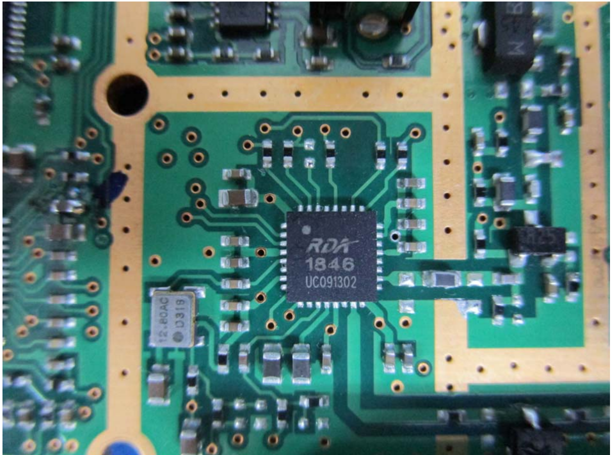
(26) EUT Photo (MB)
