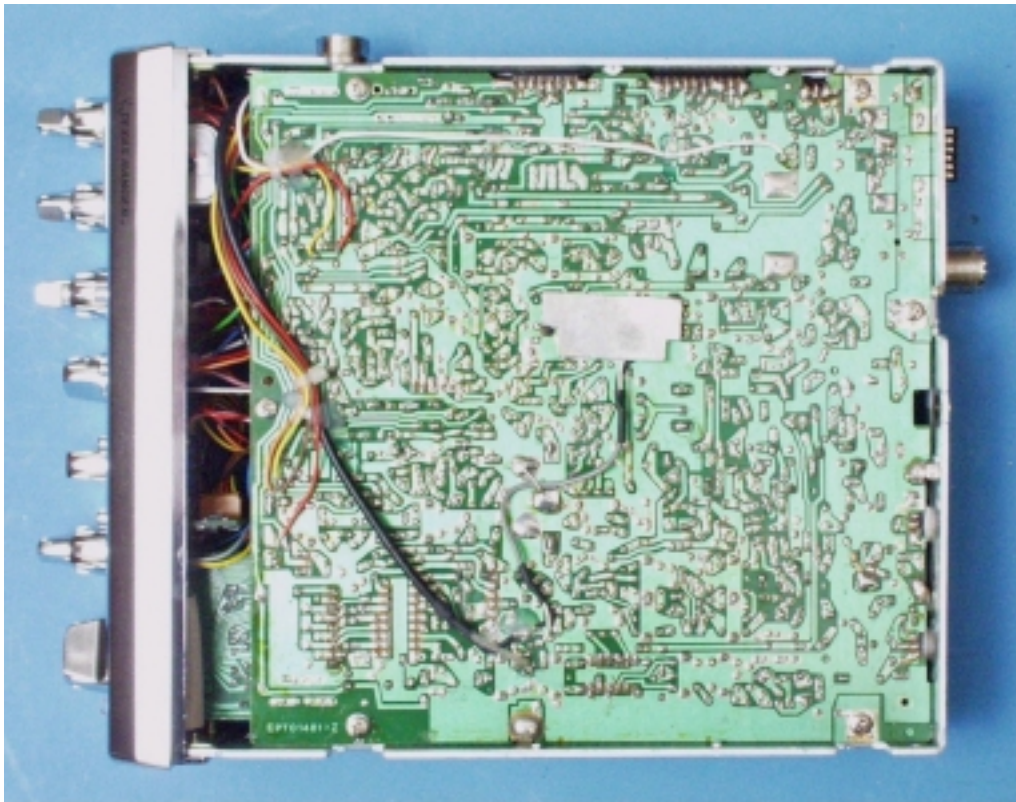
CIRCUIT BOARD, TRAC SIDE
