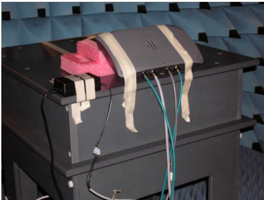
LR-6 - Radiated spurious emission 1-26 GHz
