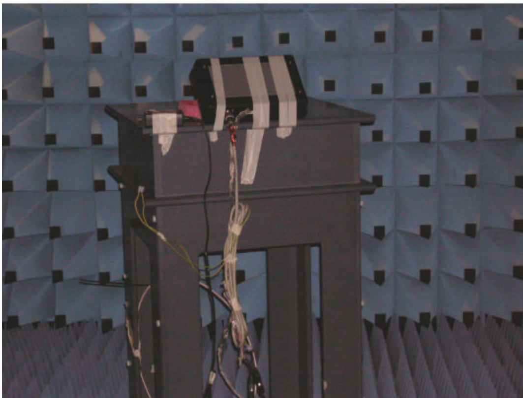
S1566 - Radiated spurious emission 1-26 GHz
