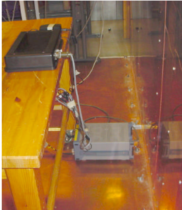
Conducted disturbance voltage 0,150-30 MHz, type S1566
