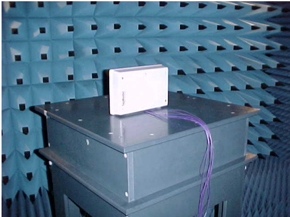
Bluetooth anechoic shielded chamber (1 – 26 GHz), type S1500
