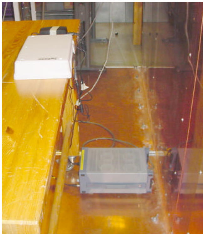
Conducted disturbance voltage 0,150-30 MHz, type S1500
