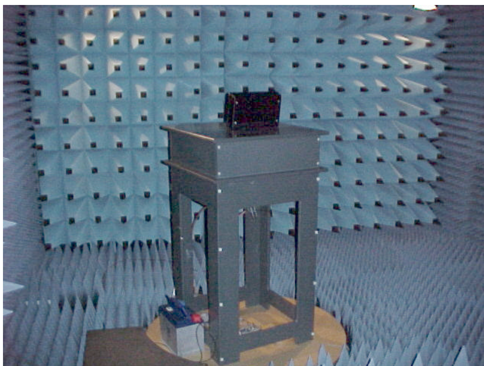
Bluetooth anechoic shielded chamber (1 – 13 GHz), type S1566
