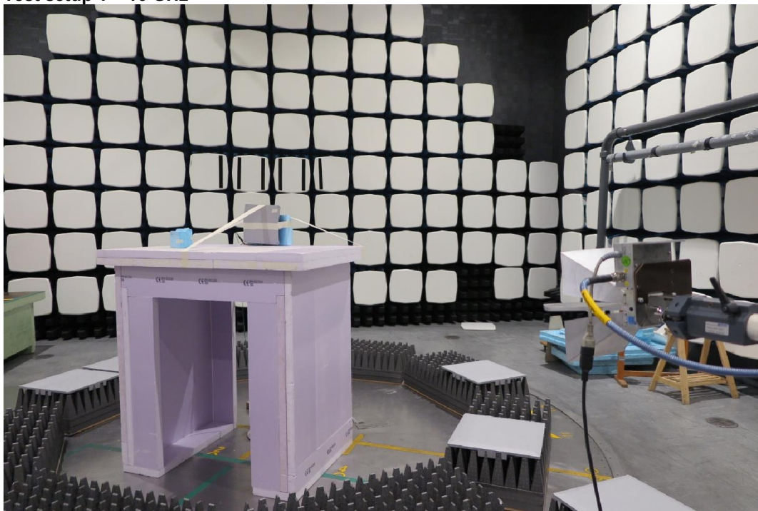
Test setup 1 – 10 GHz
