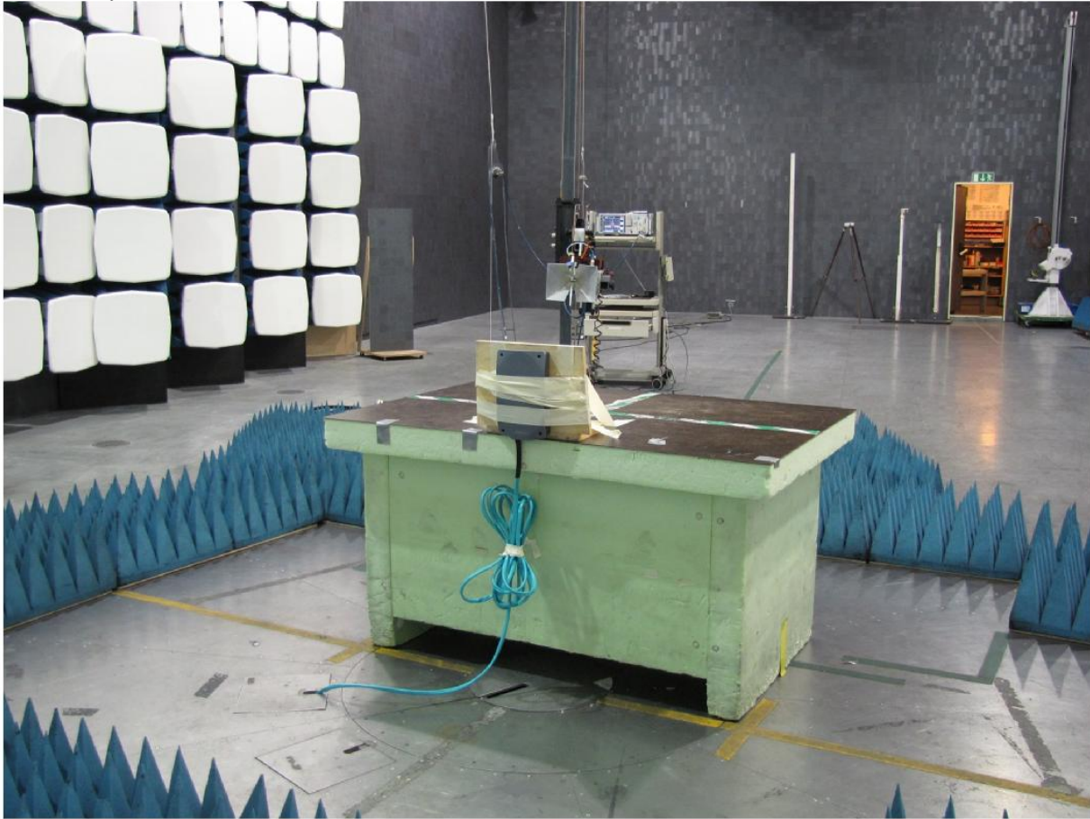
Test set up radiated emission 1GHz – 10 GHz
