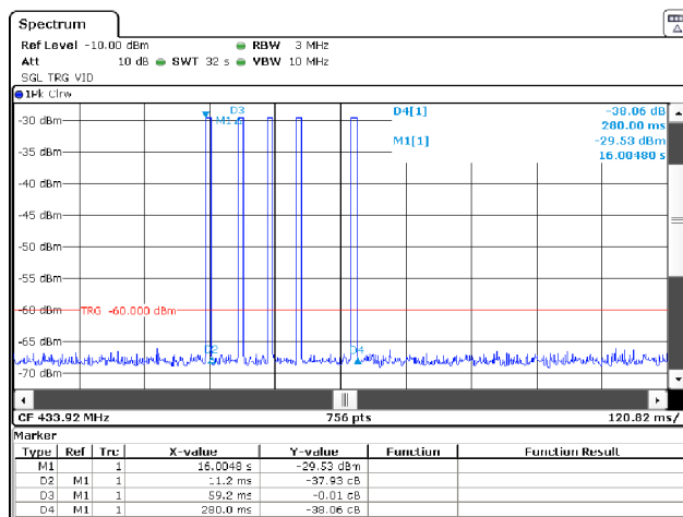
20190814-CONTI-REDI5-DUTY-PT1A-B
