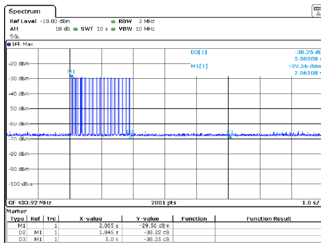
20190814-CONTI-REDI5-DUTY-MA1
