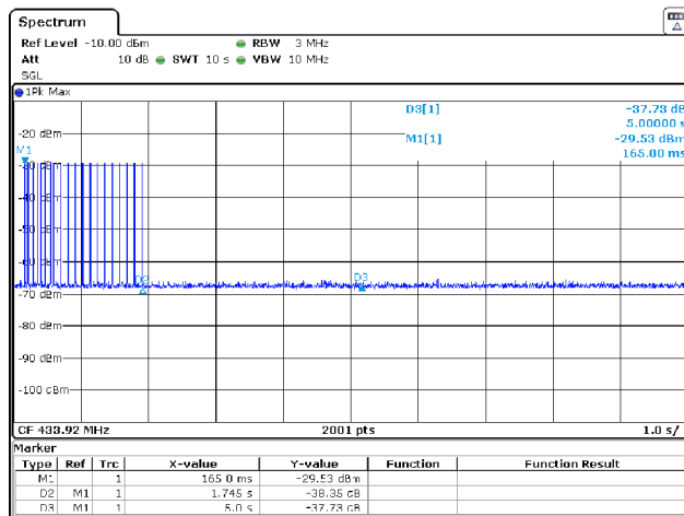
20190814-CONTI-REDI5-DUTY-MA3
