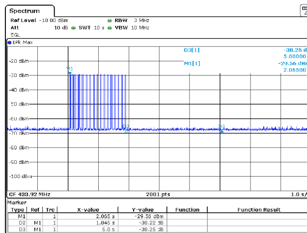
20190814-CONTI-REDI5-DUTY-MA2
