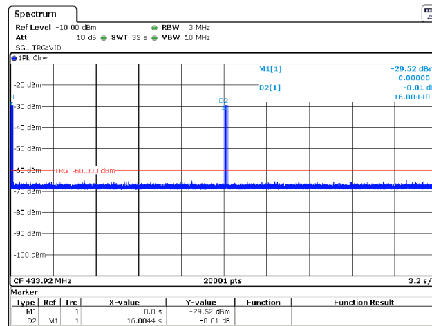
20190814-CONTI-REDI5-DUTY-PT1A-A
