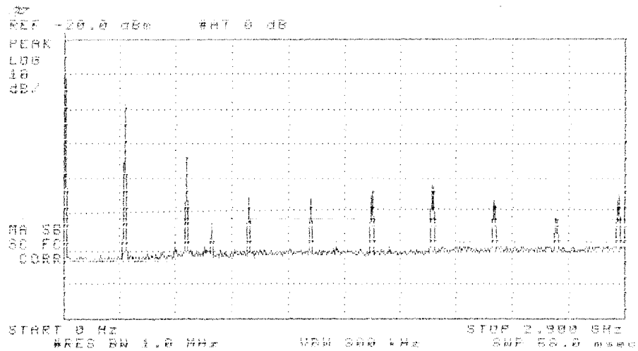
Figure 6.2. Emission spectrum of the DUT (pulsed emission). The amplitudes are only indicative (not calibrated).
