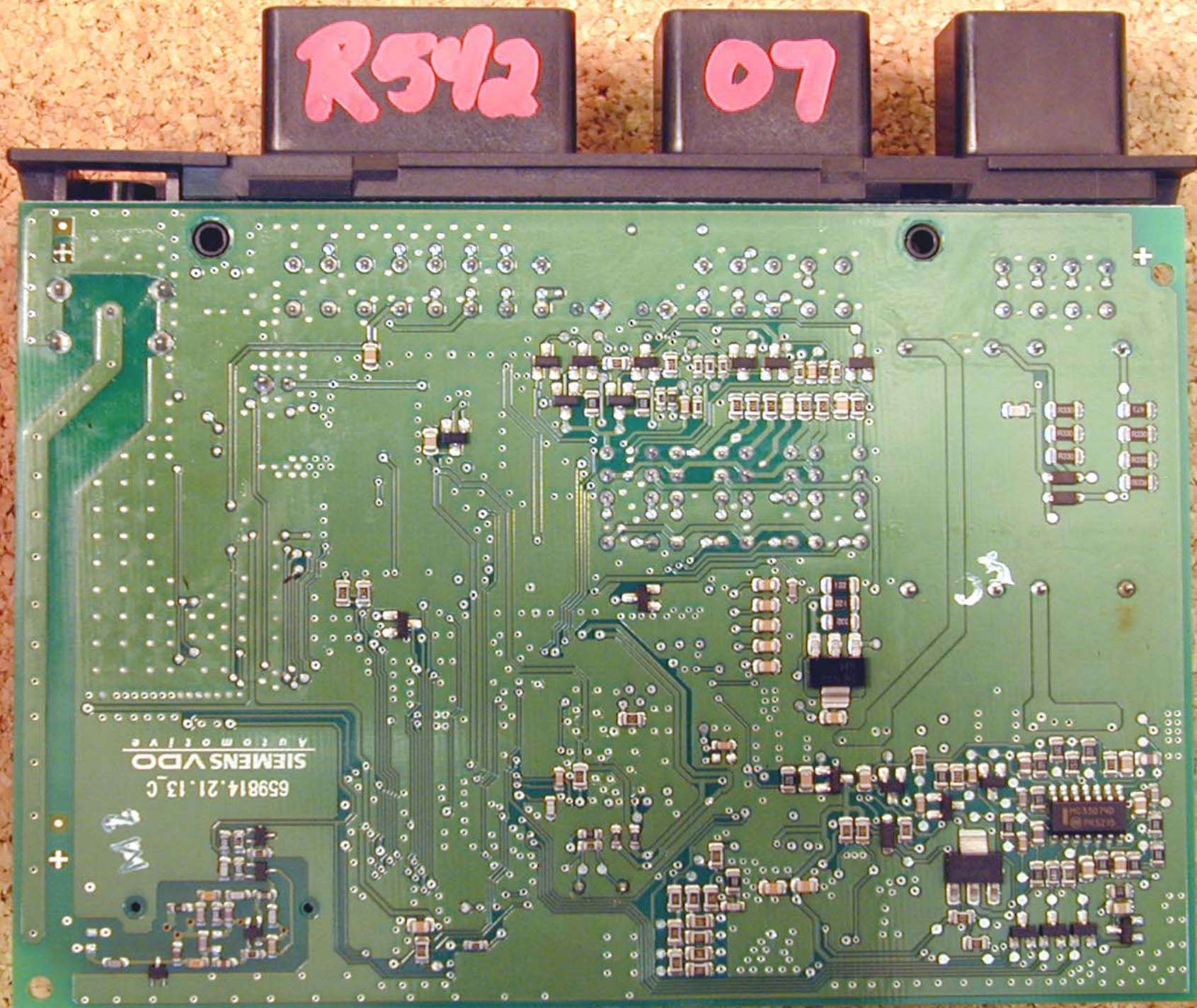
PCB (bottom)
