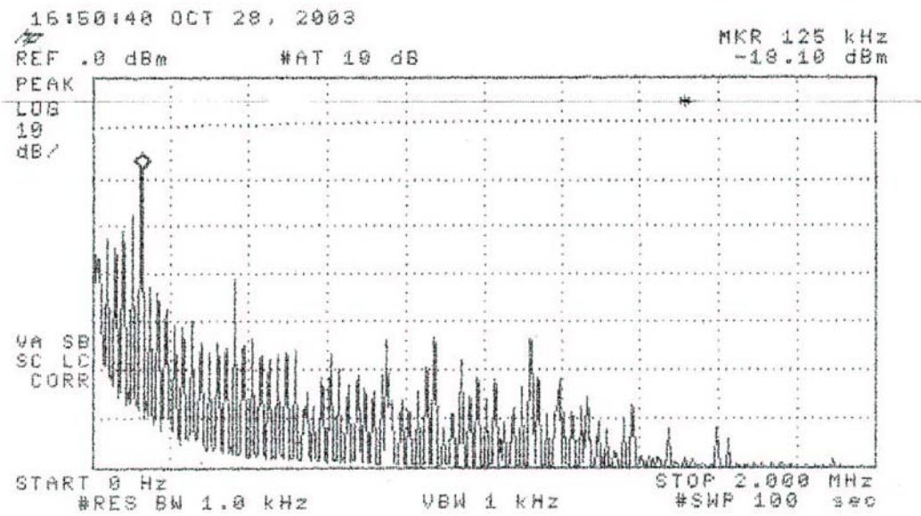
Figure 6.2. Emission spectrum of the DUT. The amplitudes are only indicative (not calibrated).
