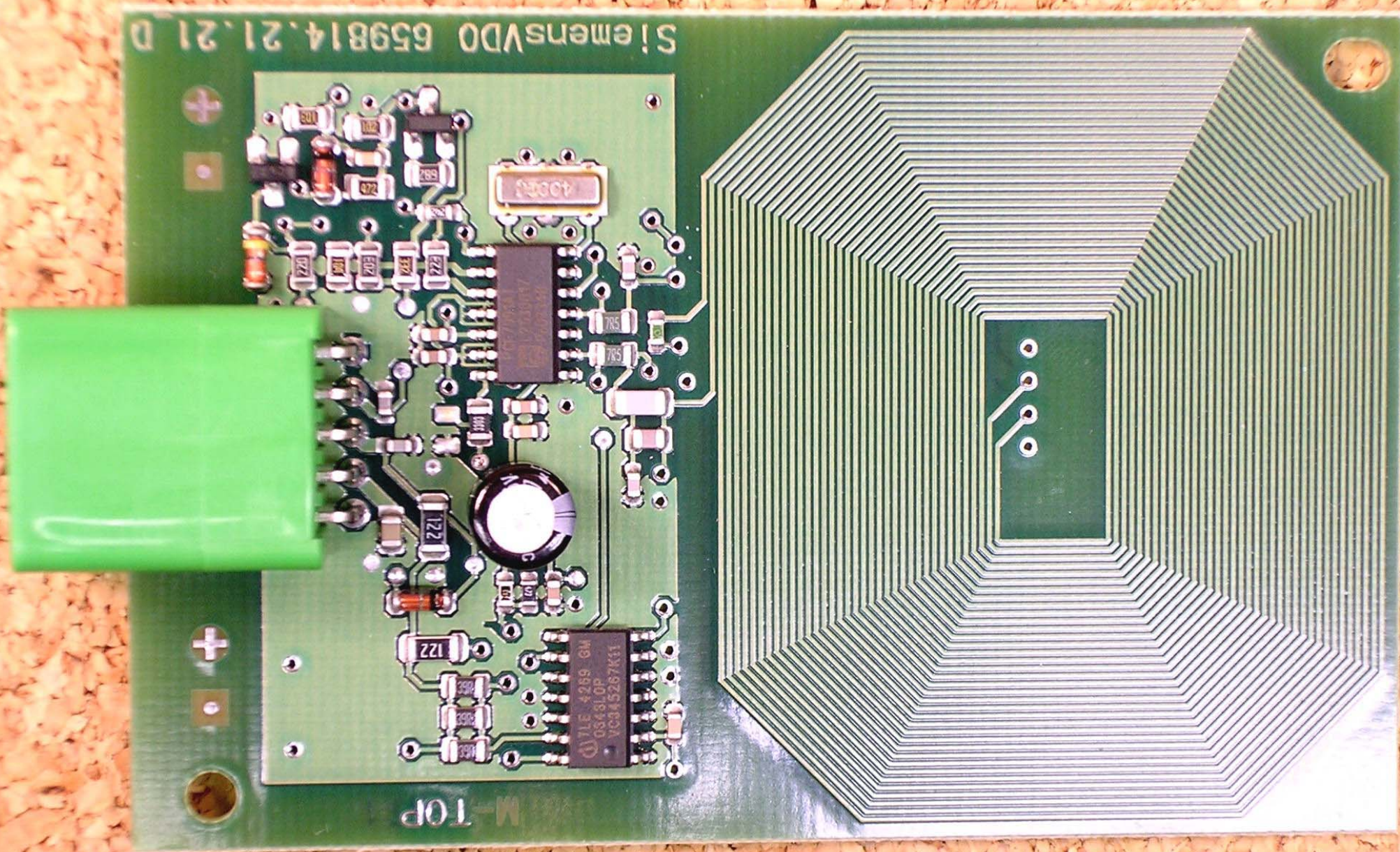
PCB (top)
