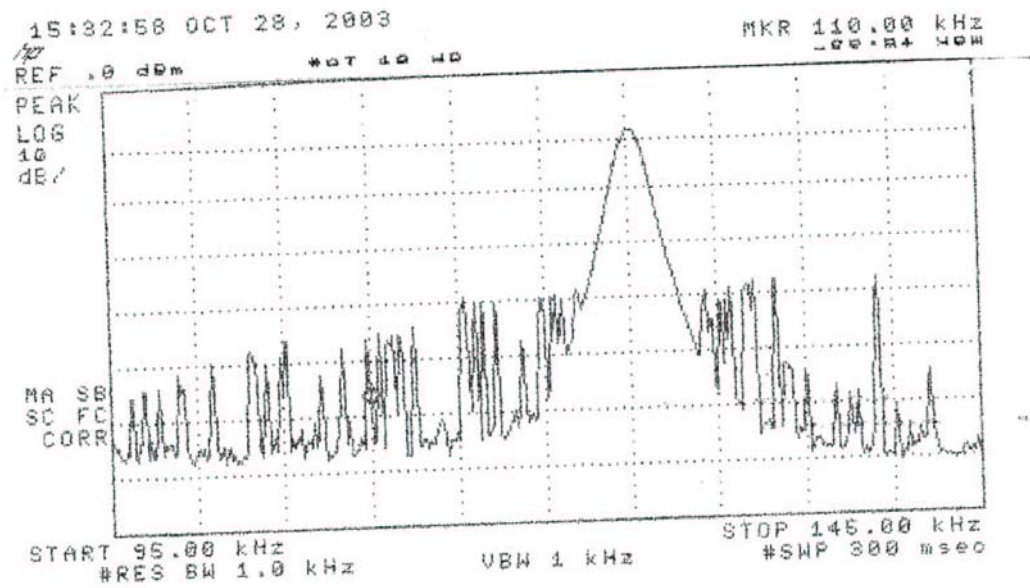
Figure 6.3. Measured bandwidth of the DUT. (pulsed)
