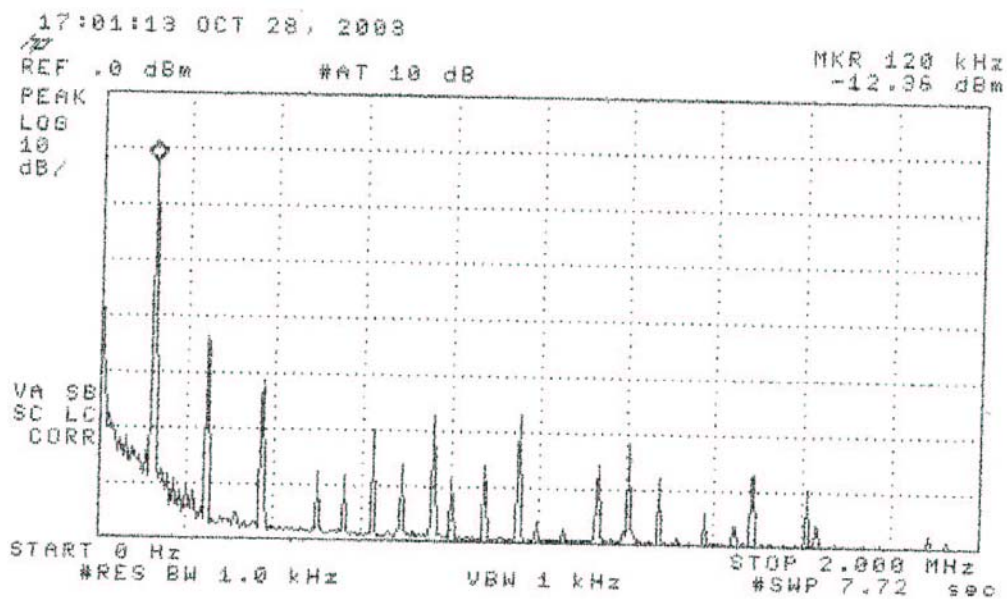
Figure 6.2. Emission spectrum of the DUT. The amplitudes are only indicative (not calibrated).
