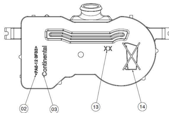
LASER MARKING - COVER SIDE (BOTTOM VIEW) Scale: 3:1
