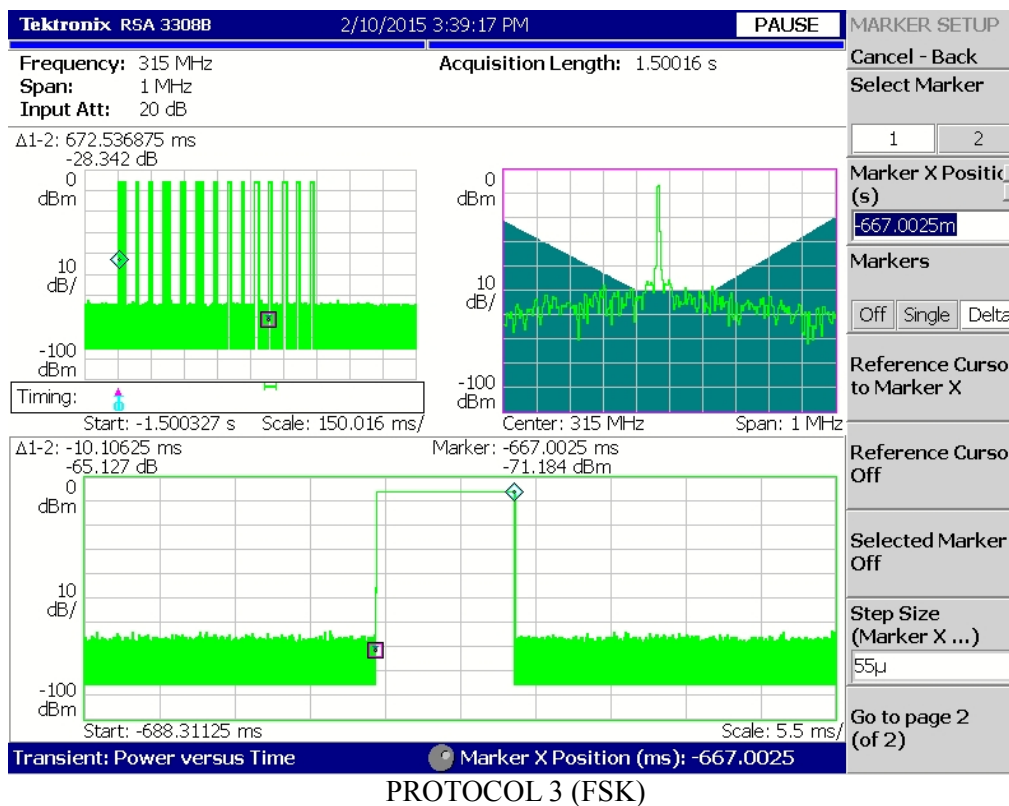
Figure 5(b): Fundamental Emission Pulsed Operation.
