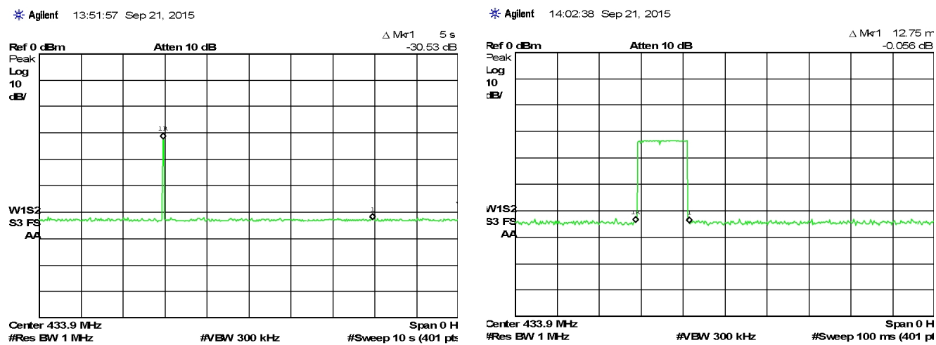
Figure 5(c): Fundamental Emission Pulsed Operation.
