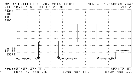
Figure 5: Fundamental Emission Pulsed Operation.
