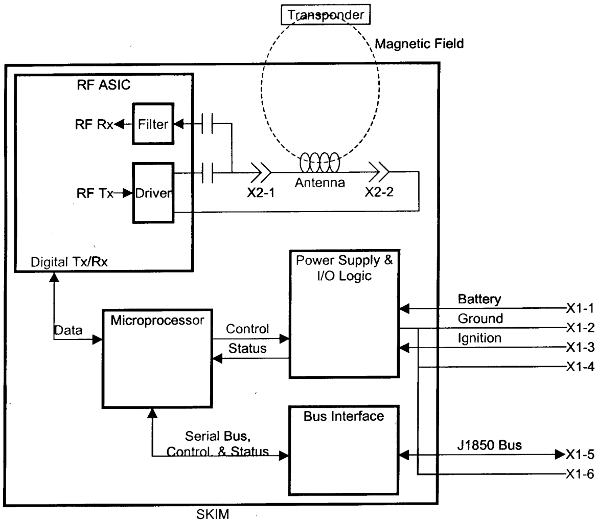
DaimlerChrysler SKIM Internal Block Diagram
