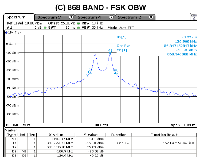
Figure 6(a): Fundamental Emission Bandwidth.
