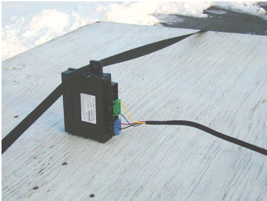
Close-up on the DUT on OATS
