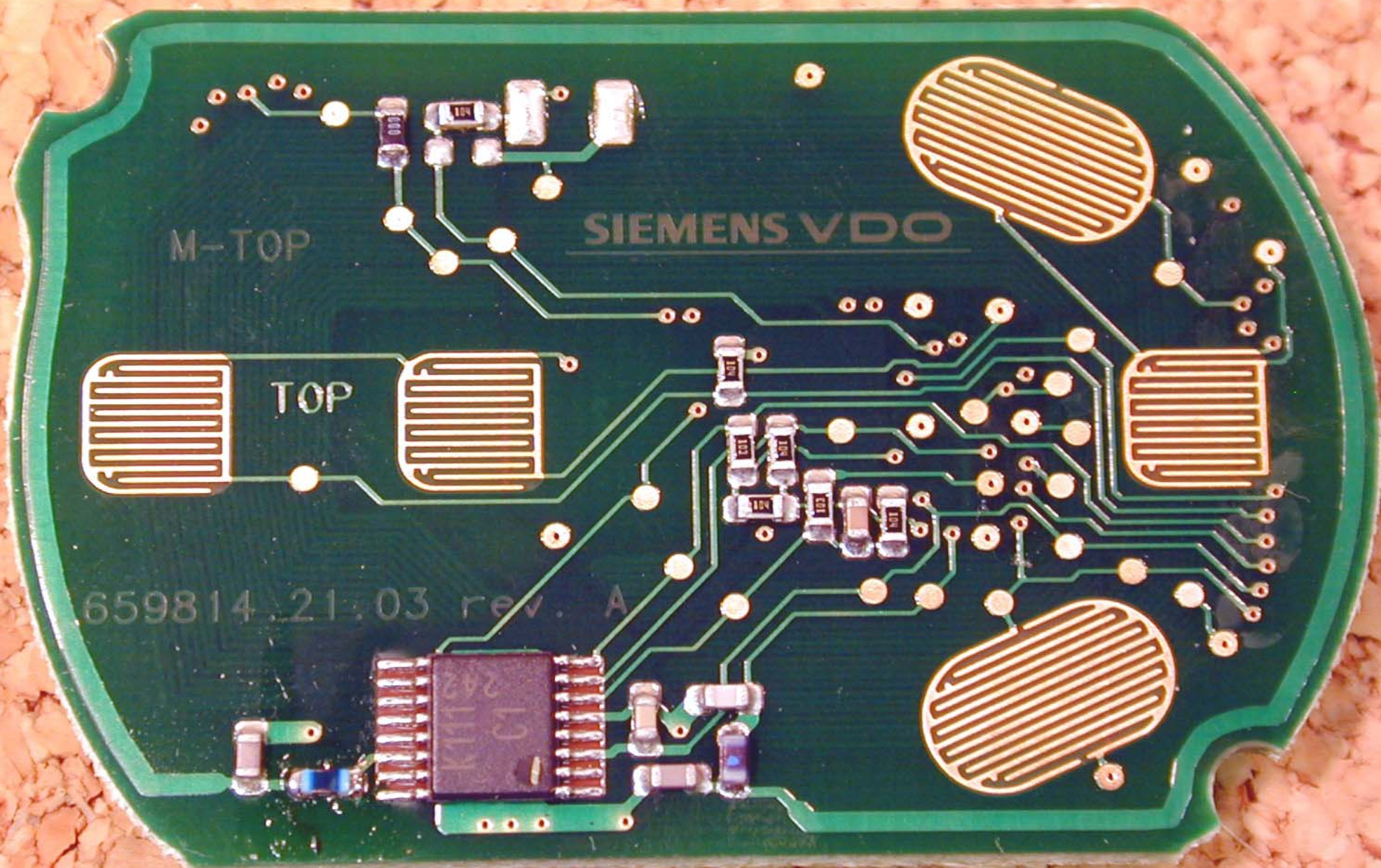
PCB (top)
