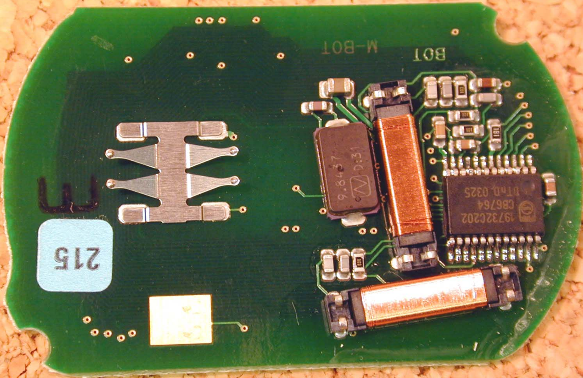
PCB (bottom)
