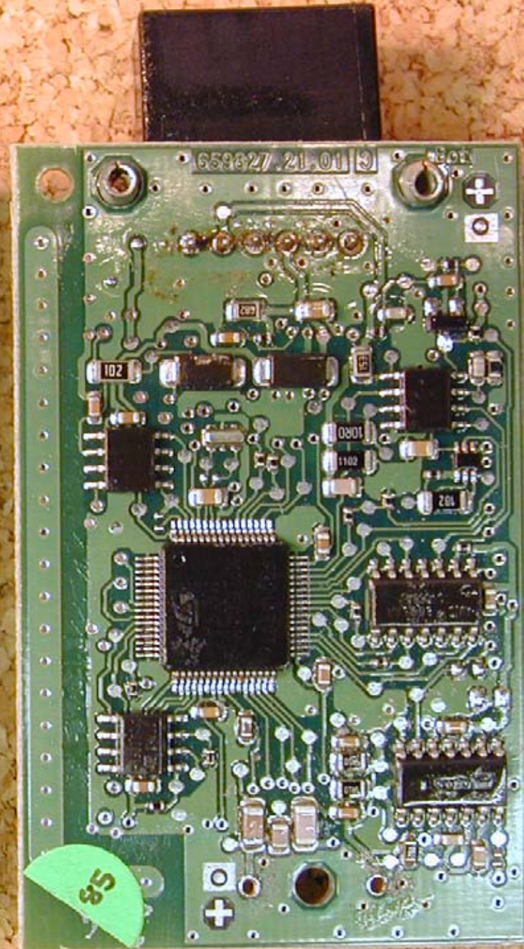
5WY7385 PCB (bot)
