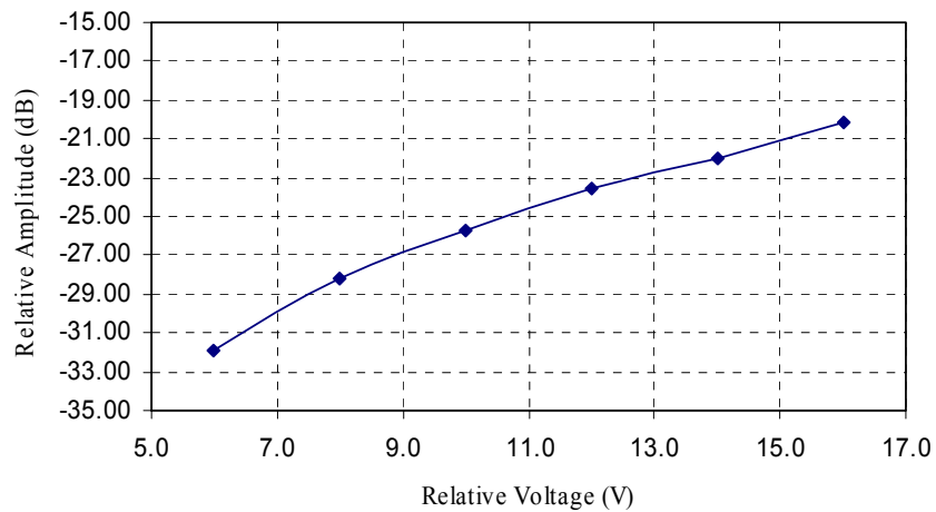
Figure 6.4. Relative emission at 135 kHz vs. supply voltage.
