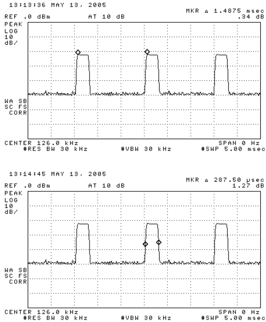
Figure 6.1. Transmission modulation characteristics.
