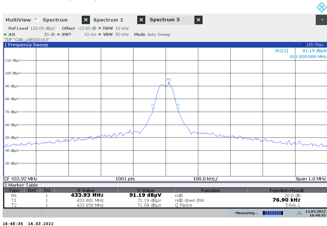
Plot No. 42: 20 dB Bandwidth, PASE, UNLOCK + TRUNK
