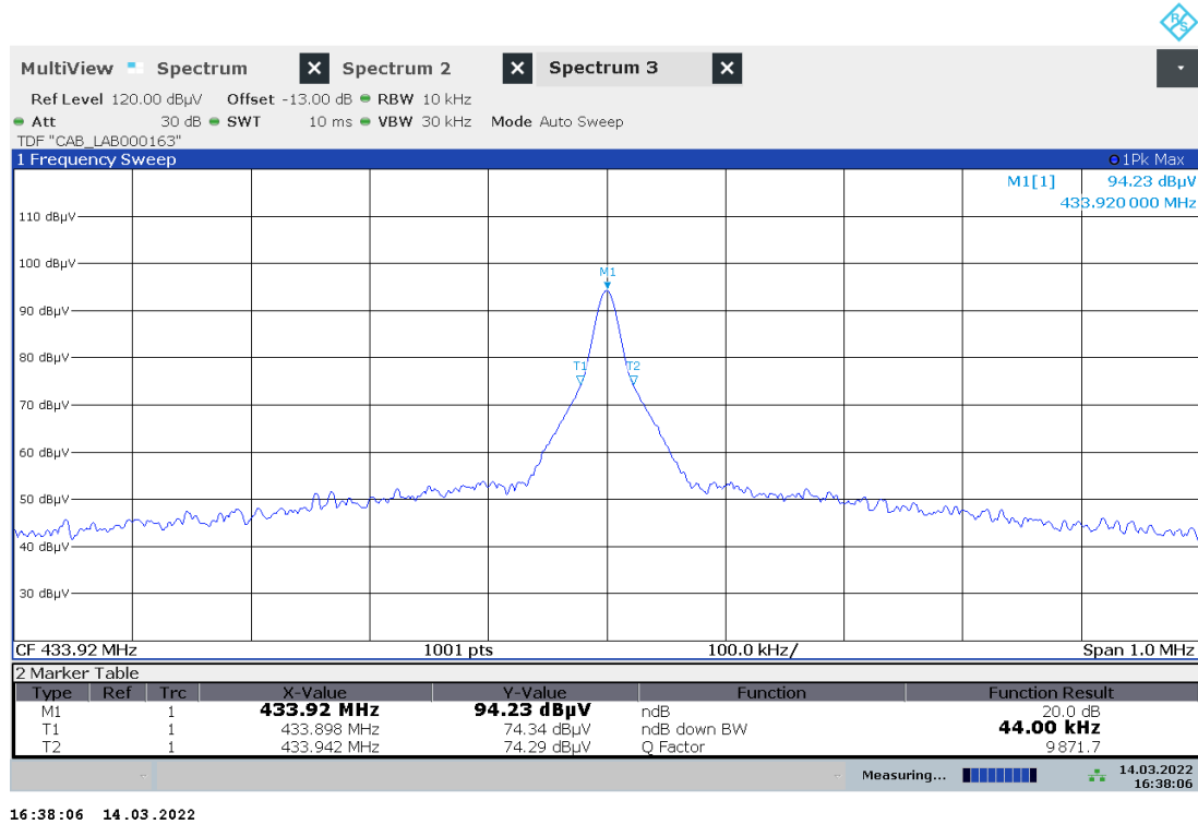
Plot No. 37: 20 dB Bandwidth, RKE, LOCK
