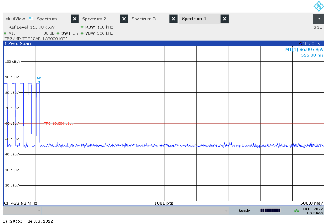
Plot no. 27: Transmission time, RKE, TRUNK
