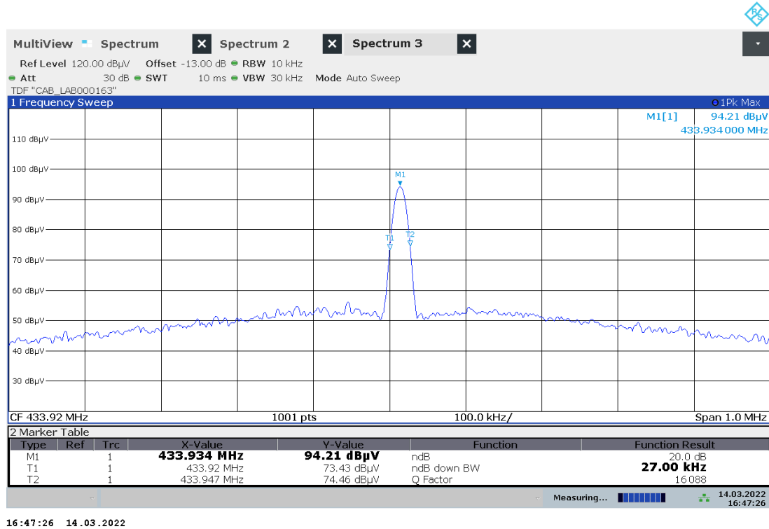
Plot No. 41: 20 dB Bandwidth, PASE, LOCK + TRUNK
