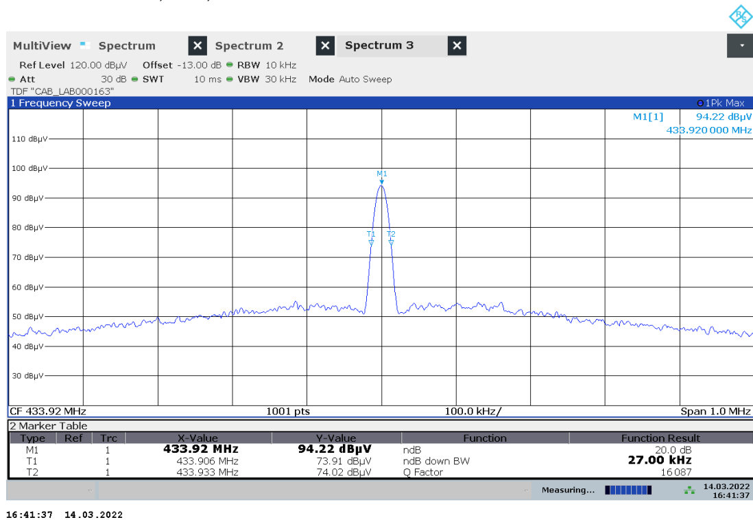
Plot No. 38: 20 dB Bandwidth, RKE, UNLOCK
