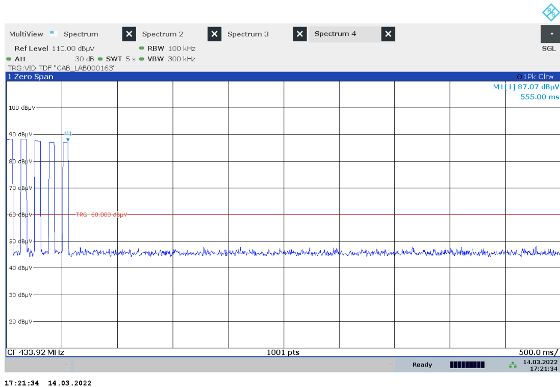
Plot no. 28: Transmission time, RKE, LOCK + UNLOCK
