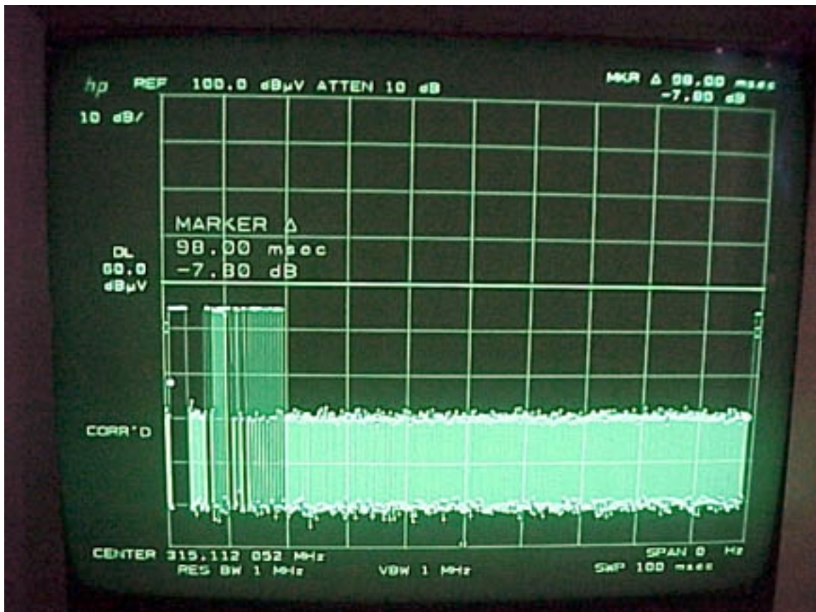
98 mS Pulse Train
