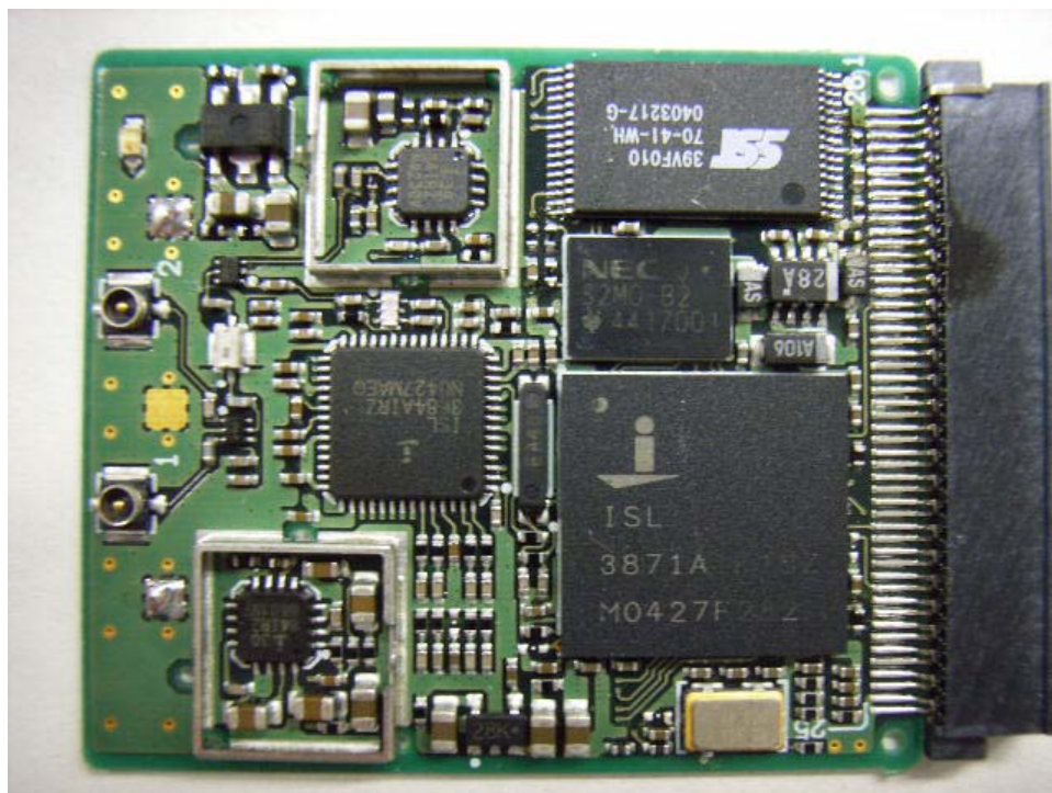
Front View without Cover
