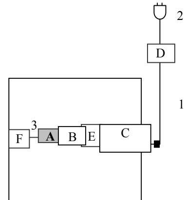
Top View (Radiated emission)
