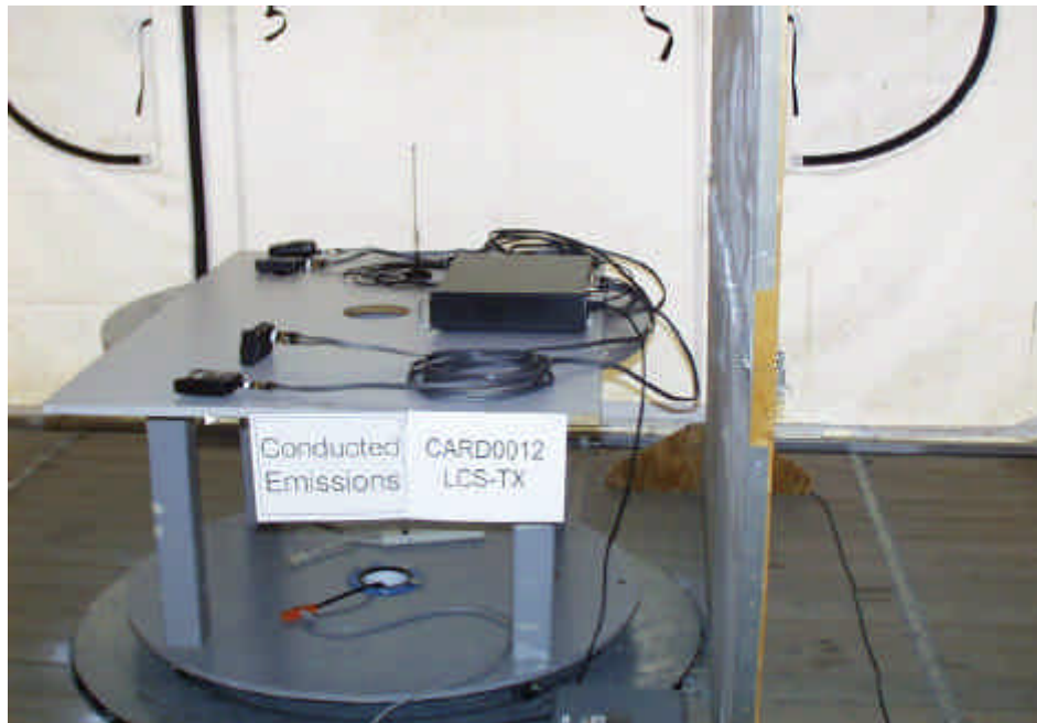
Conducted Emissions, Test Setup.
