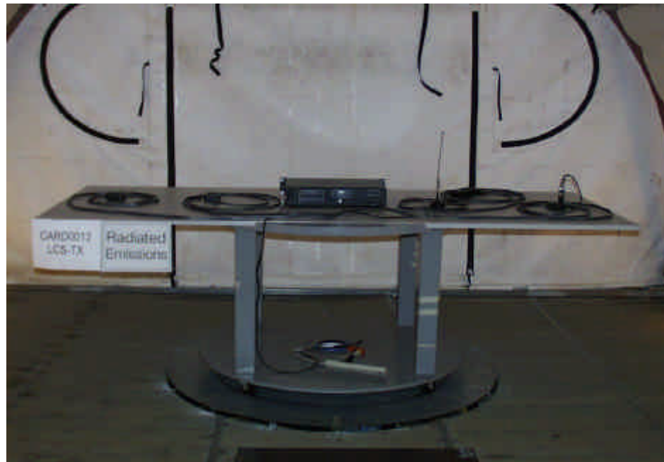
Radiated Emissions, Test Setup.
