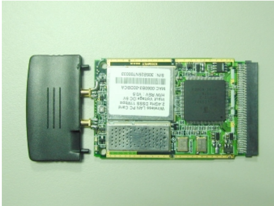
Photo 1: Outlook of XI-305M (with Antenna 1)
