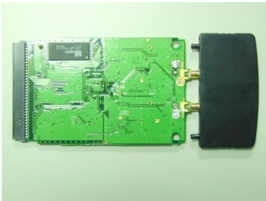
Photo 2: Outlook of XI-305M (with Antenna 1)
