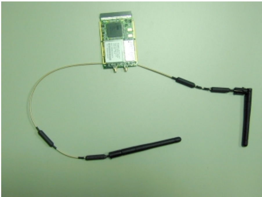
Photo 8: Outlook of XI-305M (with Antenna 3)
