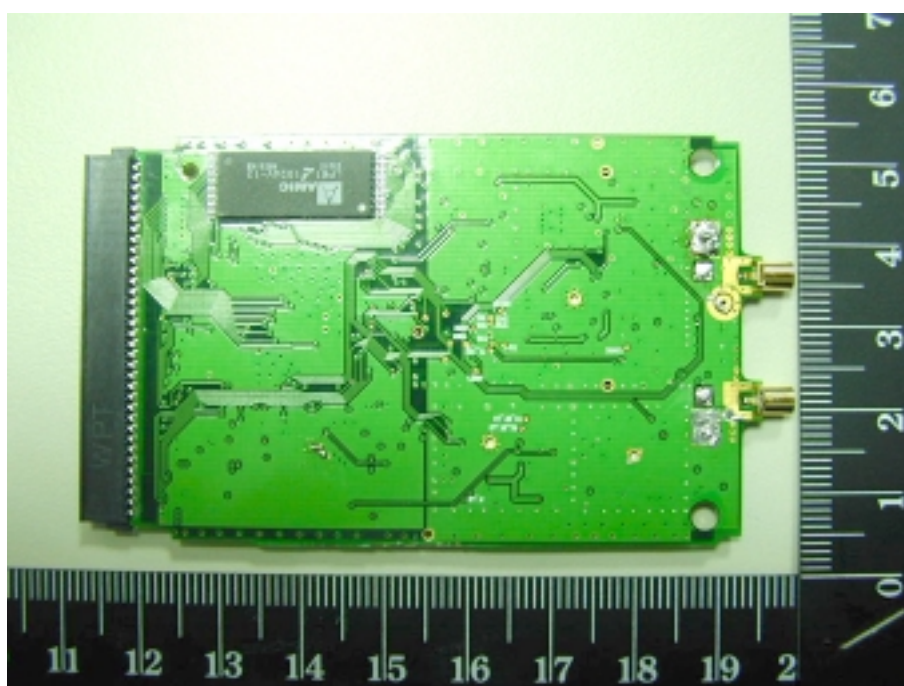
Photo 2: Internal photo of module
