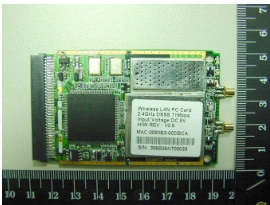
Photo 1: Internal photo of module
