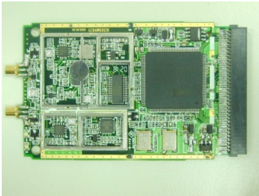
Photo 3: Internal photo of module
