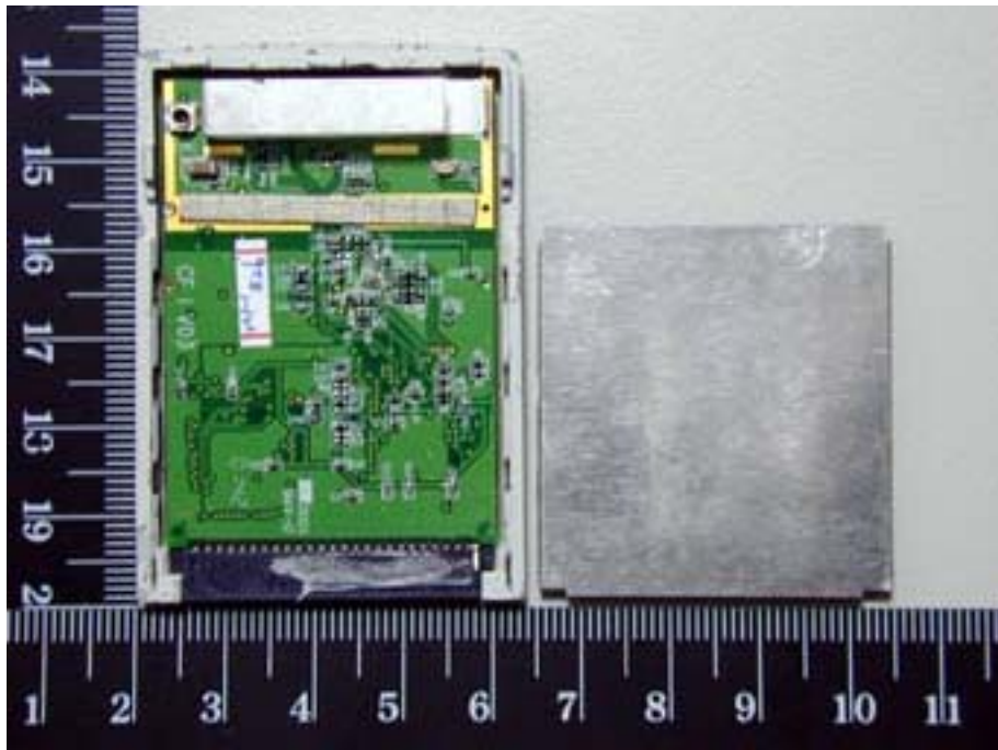
Photo 2: Inner view
