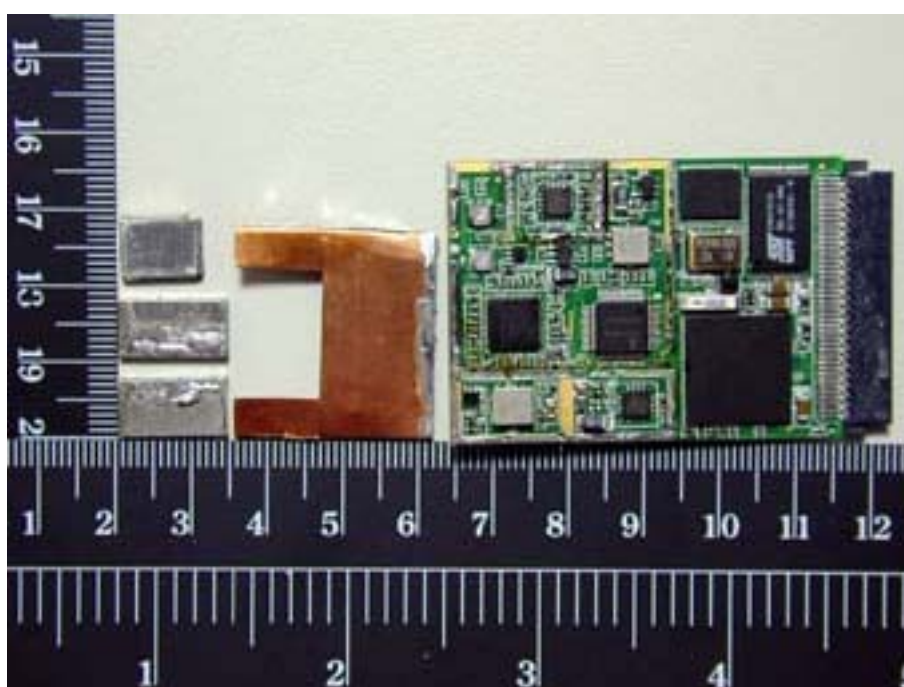
Photo 6: Inner view
