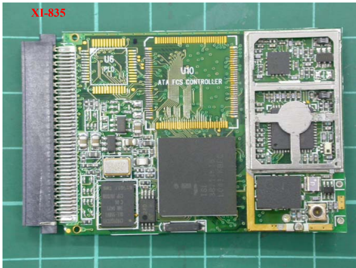
Photo 2: Interior photo of EUT
