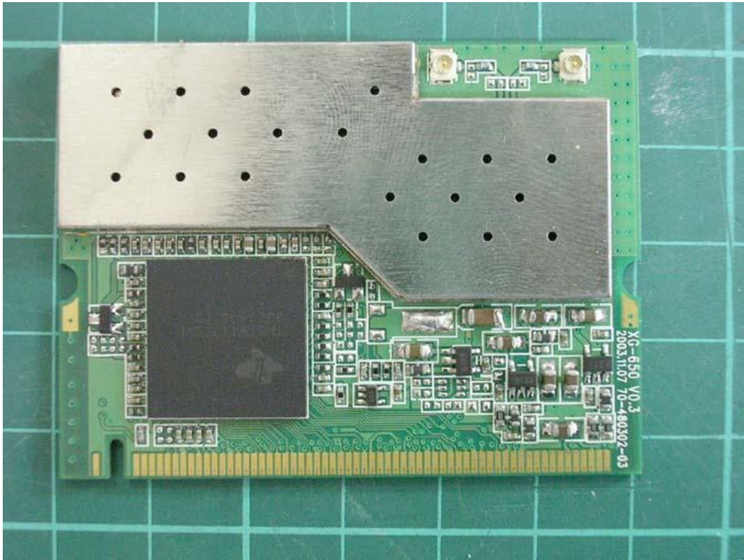
Photo 1: External photo of EUT
