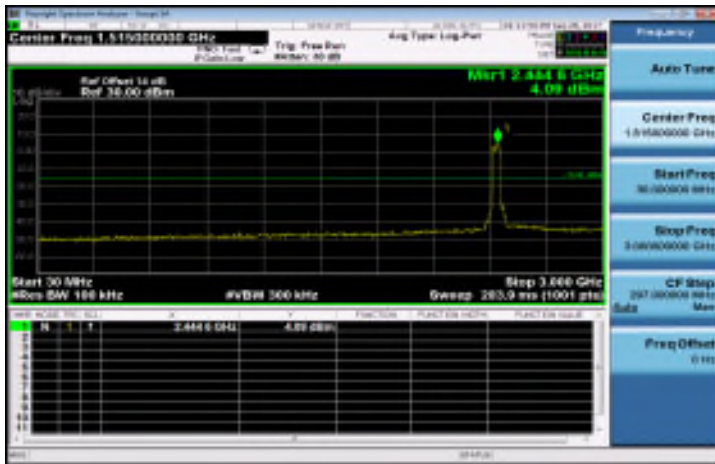
802.11n_HT40: Spurious Emission Test Data CH-Mid (MIMO)
