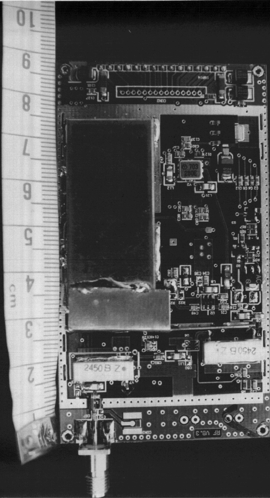
Disassembled View of RF Module-1(Front Side)
