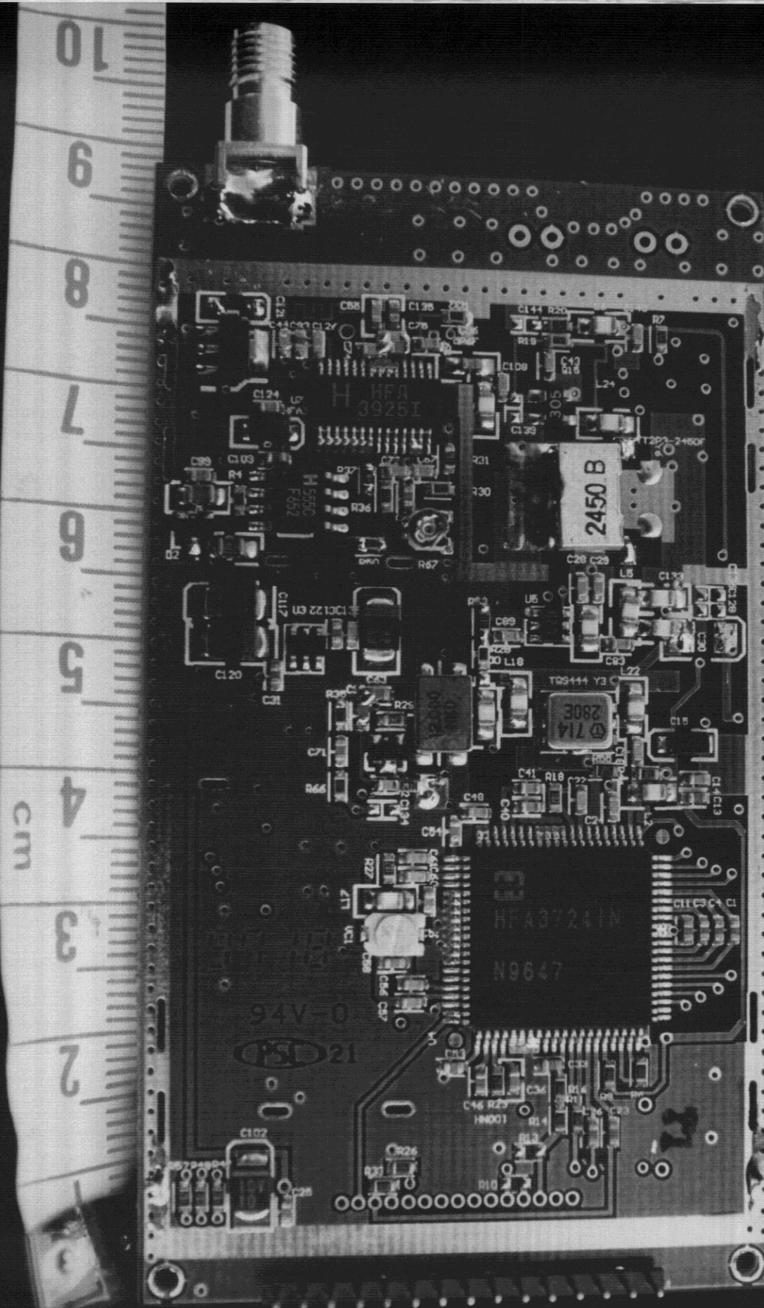
Disassembled View of RF Module (Back Side)
