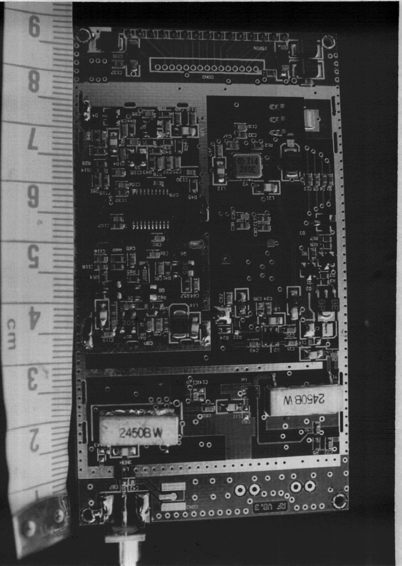
Disassembled View of RF Module-2(Front Side)
