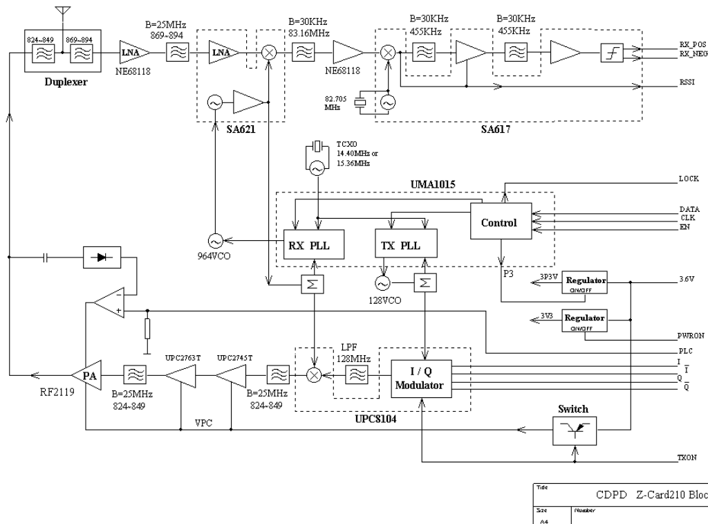
Figure 4-2 Z-Card 210 Radio Block Diagram
