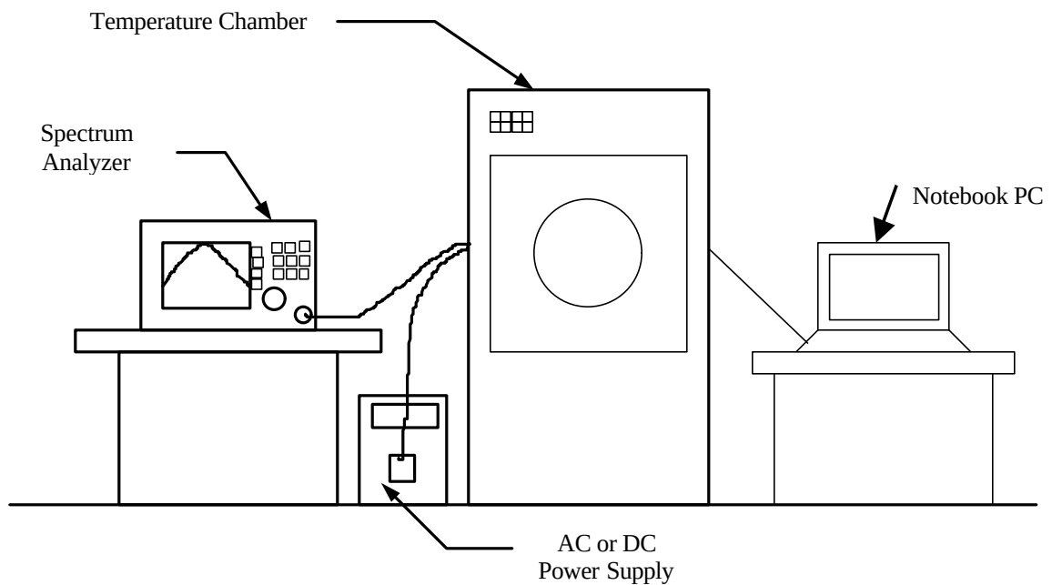
Figure 5 : Frequency stability measurement configuration
