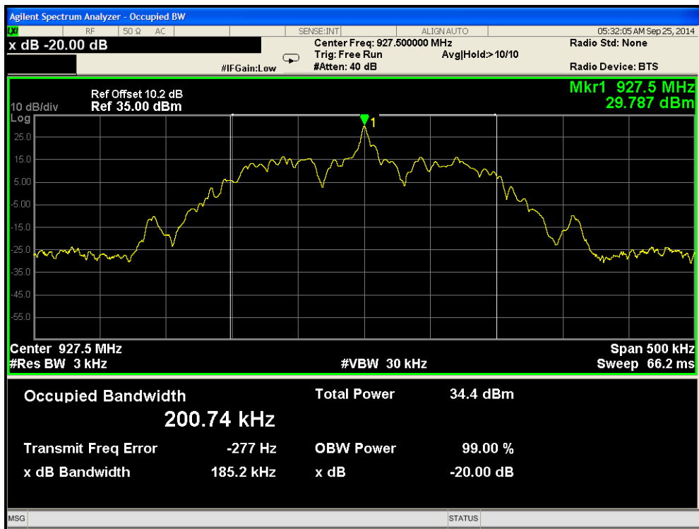
Occupied Bandwidth – Dense Mode High (higher data rate)
