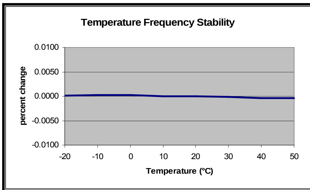
Plot 4-1: Temperature Stability
