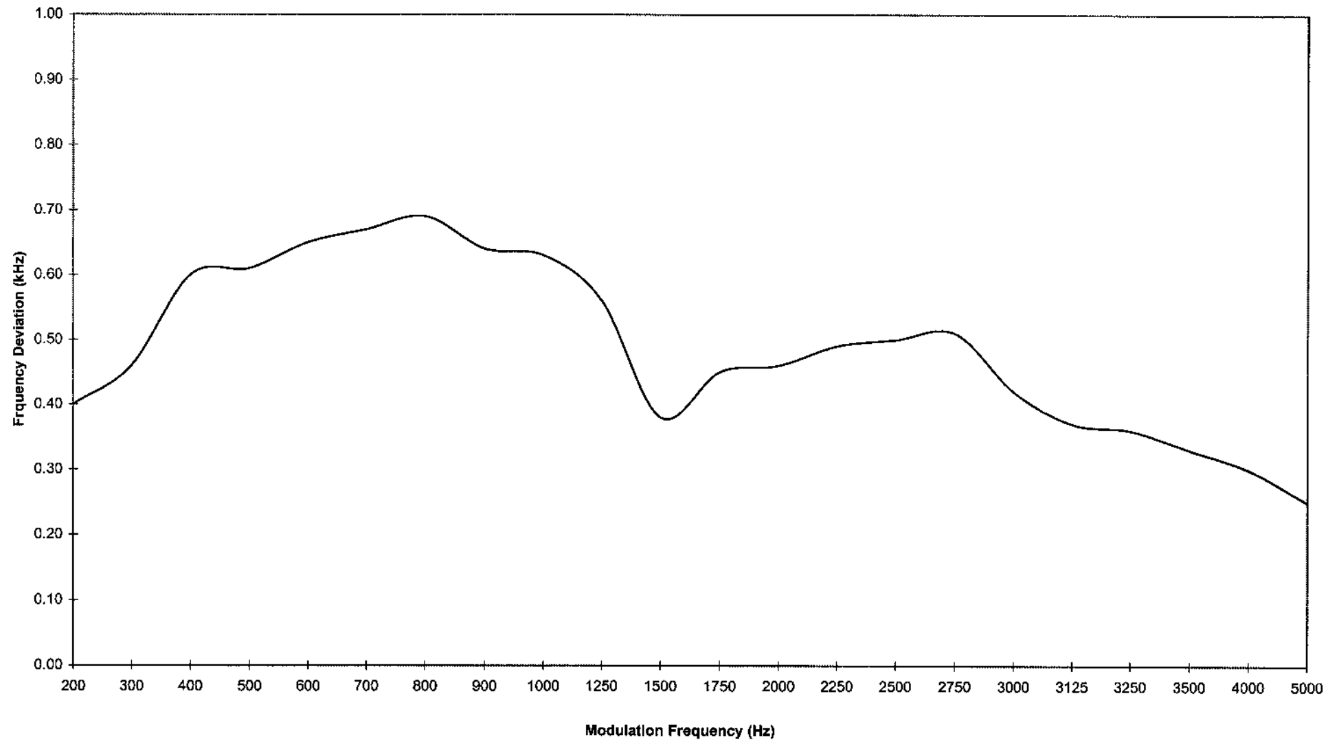
Modulation Frequency Response
