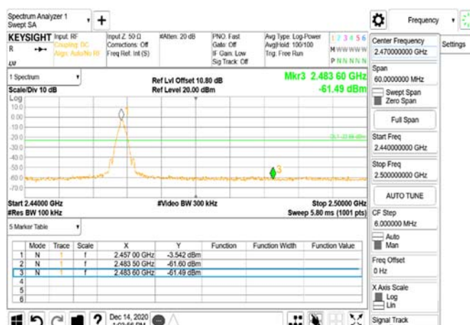
Band Edge__ANT+_High Channel
