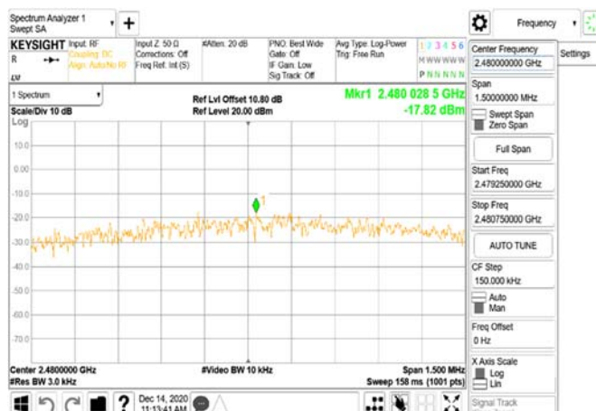
Power Density_BLE_2M_HighCH39-2480
