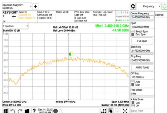
Power Density_BLE_1M_HighCH39-2480
