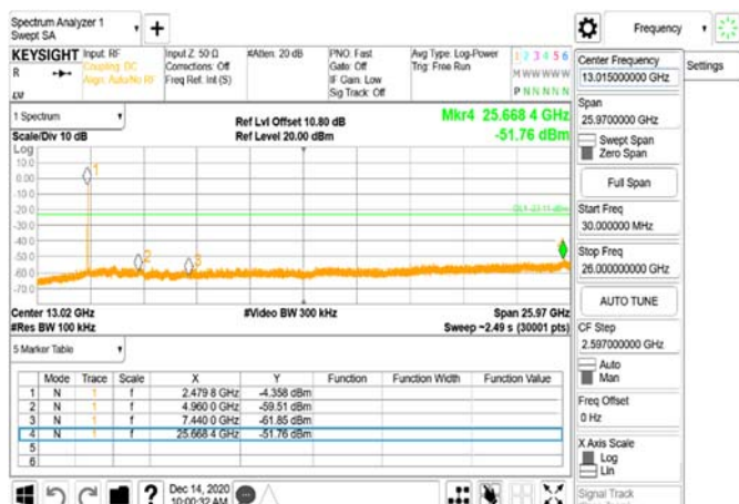
Spurious Emission_BLE_1M_HighCH39-2480
