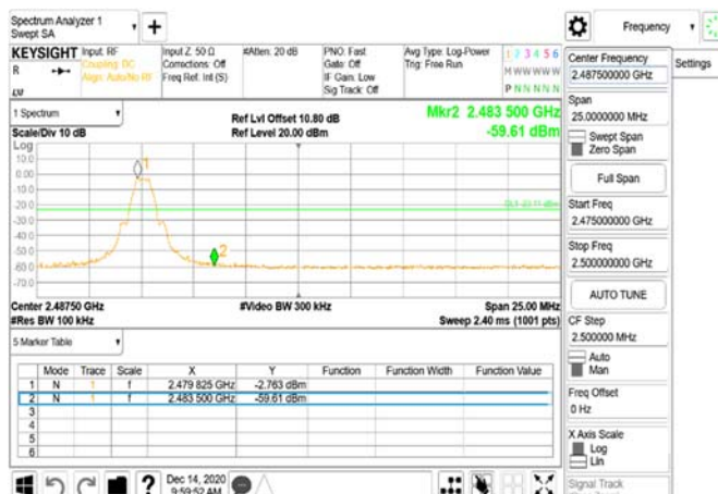
Band Edge_BLE_1M_HighCH39-2480
