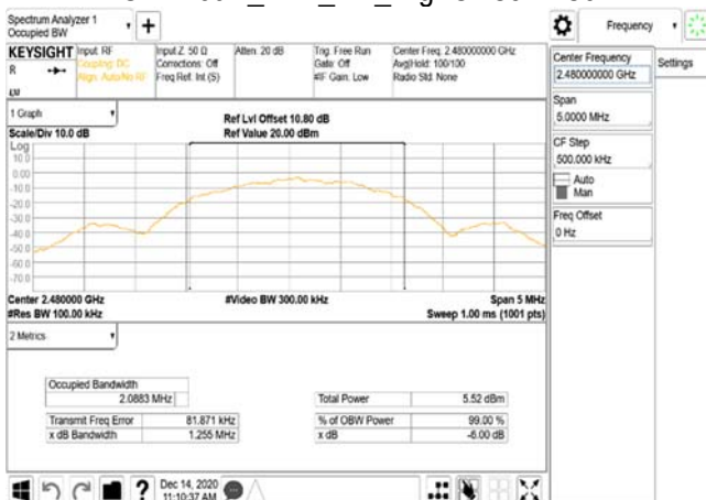
OBW 6dB_BLE_2M_HighCH39-2480
