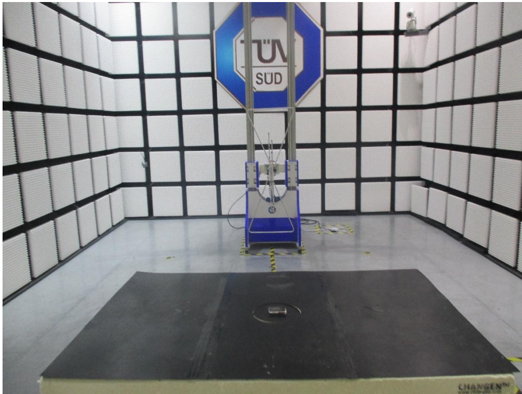
Radiated Emissions Test below 1GHz
