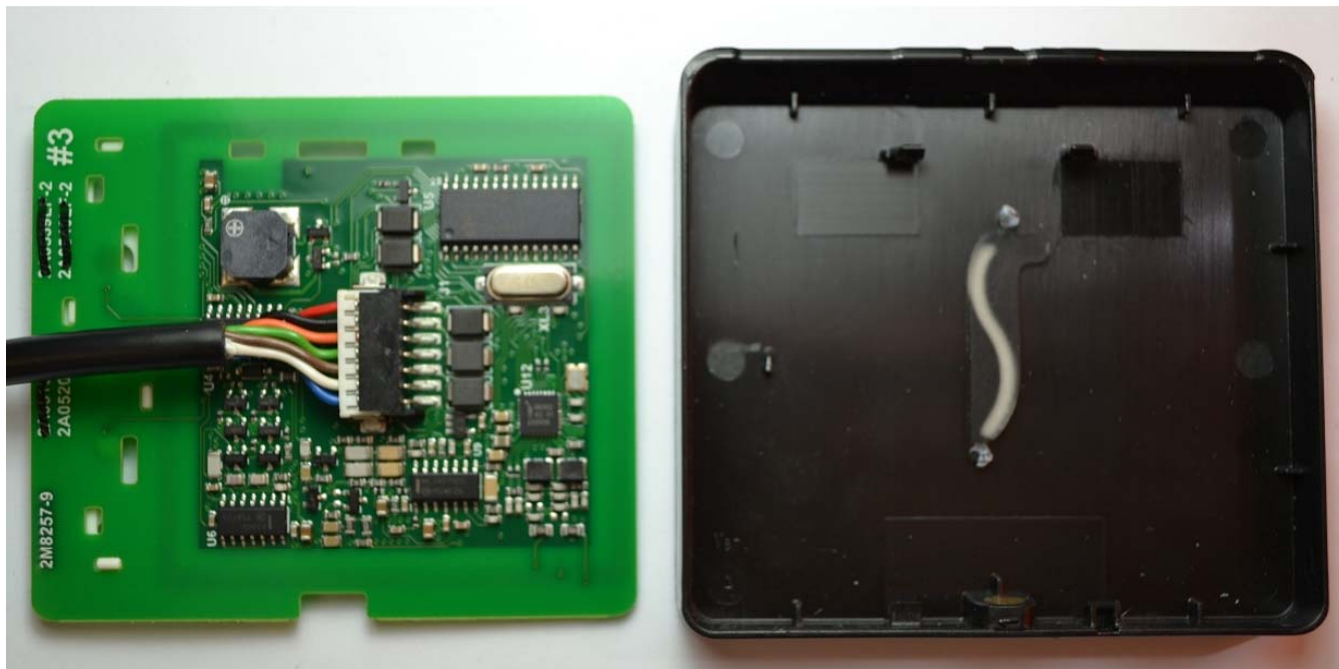
T12 Multi Tech - Front Cover and PCB Assembly
